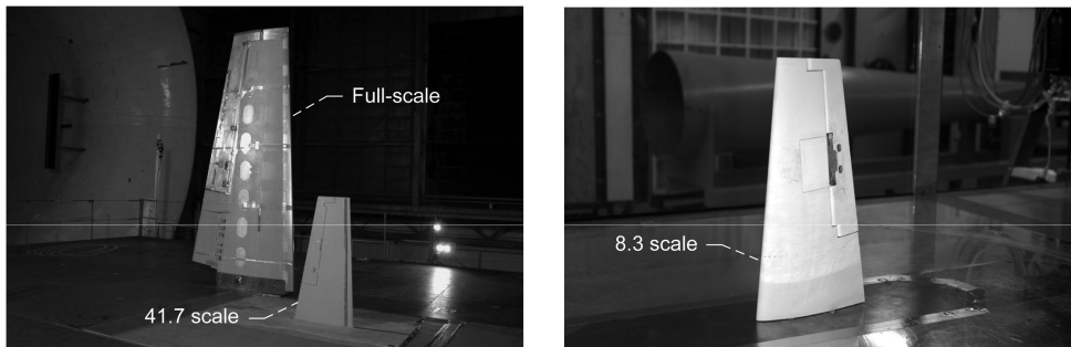
Fig. 13 Full-scale, 41.7%-scale, and 8.3%-scale business jet wing panel models.
